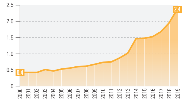
Proportion of renewable energy in primary energy in Korea; 2000~2019 (Unit: %)
