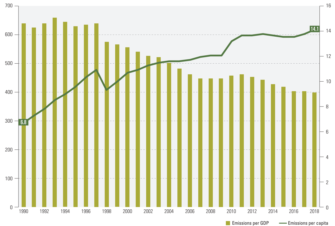
GHG emissions to real GDP and GHG emissions per capita; 1990~2018 (Unit: tonne CO 2 eq./KRW 1 billion, tonne CO 2 eq./person)
