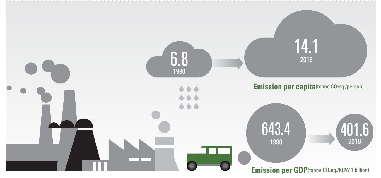
Greenhouse gas emission
