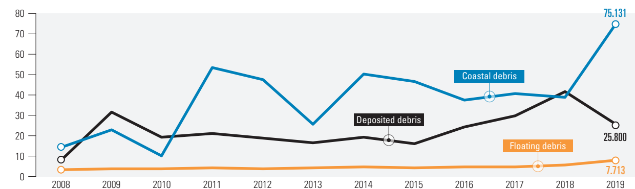
Collected marine debris by type; 2008~2019
