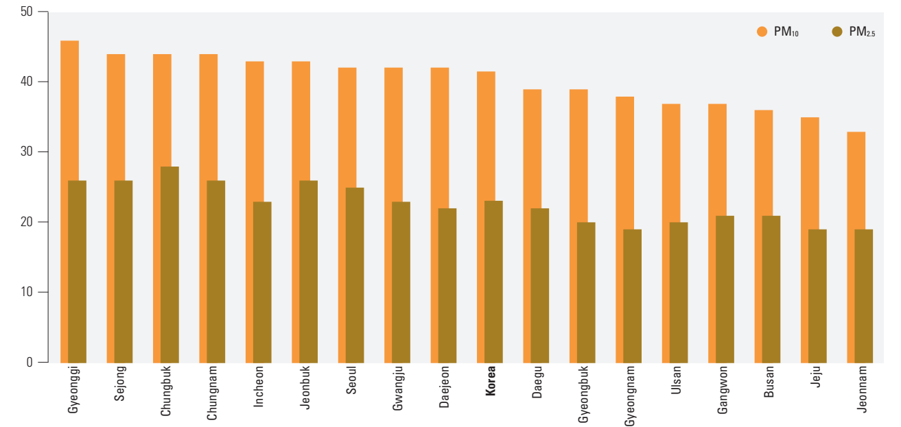
Annual average particulate matter levels by city/province; 2019 (Unit: µg/m 3 )
