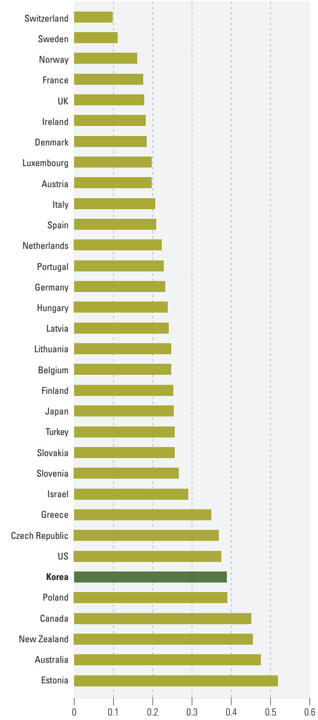
GHG emissions per GDP of OECD countries; 2018 (Unit: kgCO 2 eq./USD)
