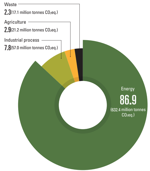
GHG emissions by sector; 2018 (Unit: %, million tonnes CO 2 eq.)
