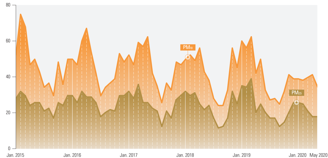
Fluctuations in particulate matter levels; Jan. 2015 ~ May 2020 (Unit: µg/m 3 )
